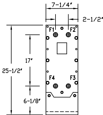
FIXED HEAD
